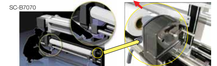
Lift lever
